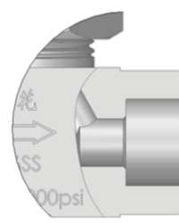
承插焊 Socket weld
